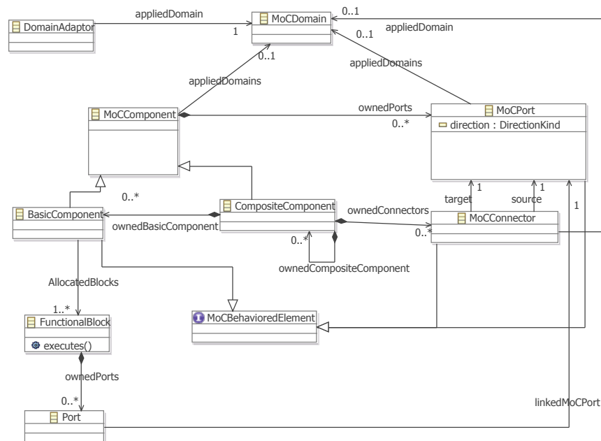
Figure 1: Excerpt of Cometa Metamodel for Architecture Description
